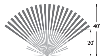
WIH-OS-LODIA Wall Mount Sensor
