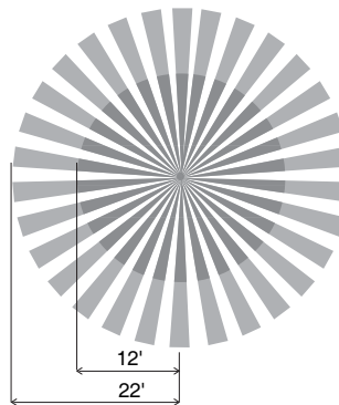
WIH-OS-OMIRL Ceiling Mount Sensor
