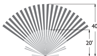
WIH-OS-LOIRWV Wall Mount Sensor
