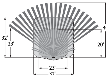
WIH-OS-LODT Wall Mount Sensor
