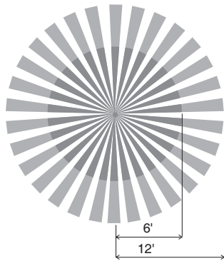
WIH-OS-OMIR Ceiling Mount Sensor
