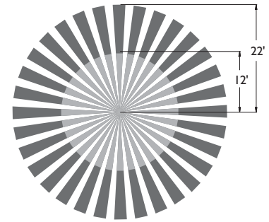
WIH-OS-OMUS2 Ceiling Mount Sensor
